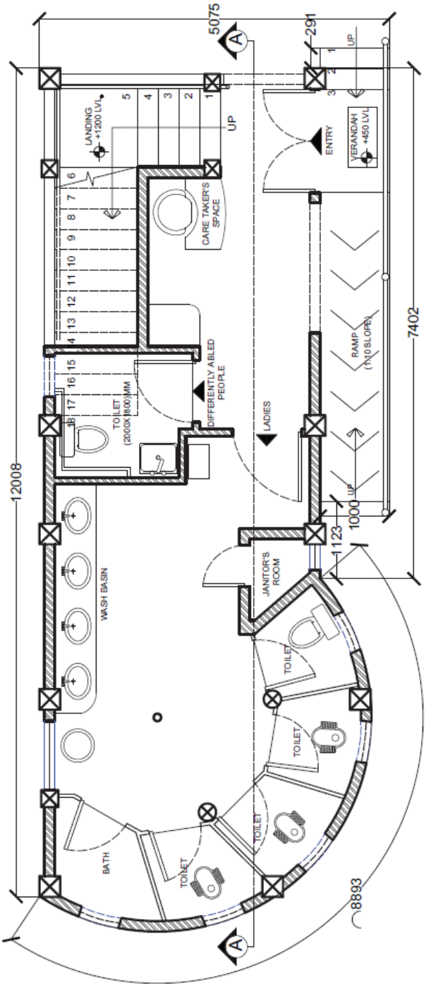
GROUND FLOOR PLAN (DIMENSION)
