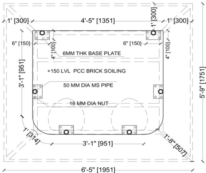
PLAN @ 150MM LVL
