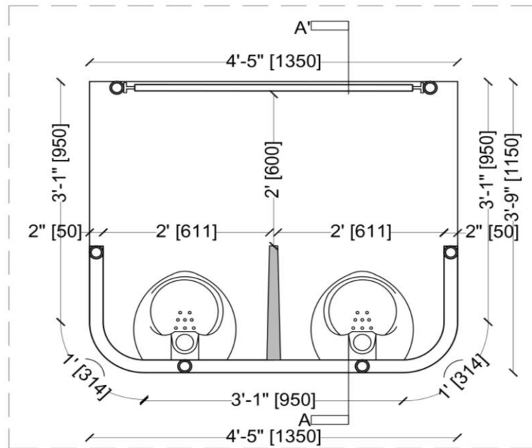
GENTS URINAL PLAN
