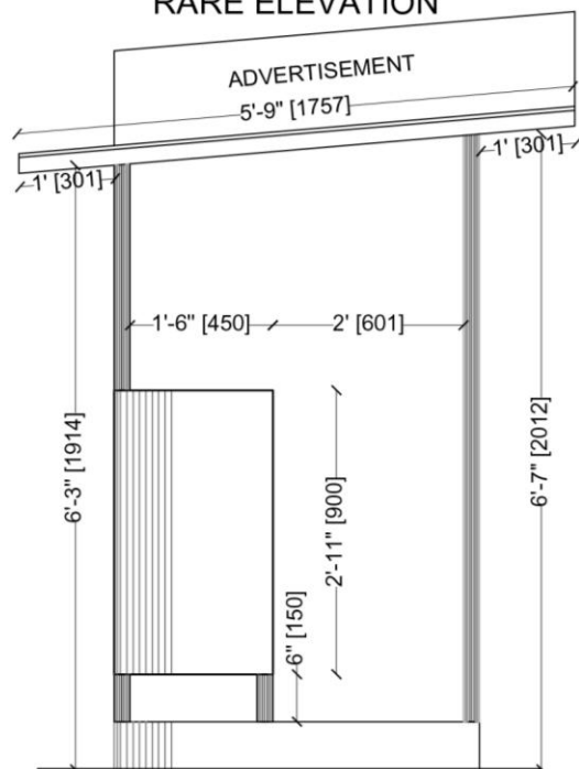
FRONT ELEVATION
