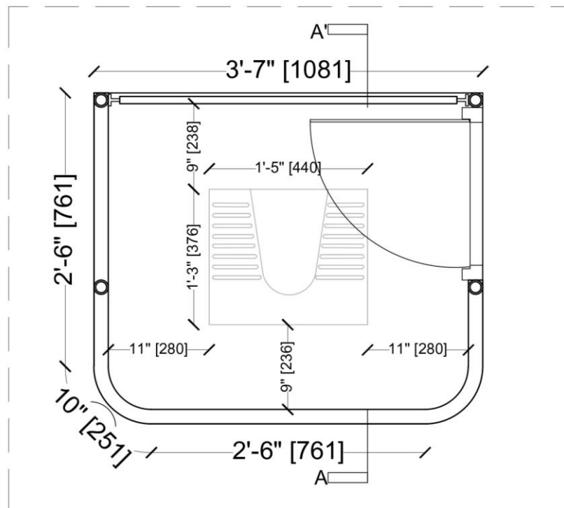
LADIES URINAL PLAN
