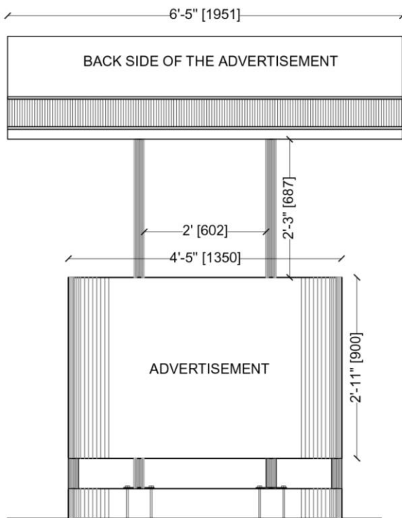
RARE ELEVATION
