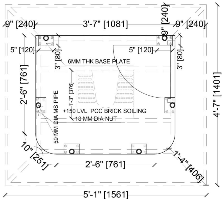
PLAN @ 150MM LVL
