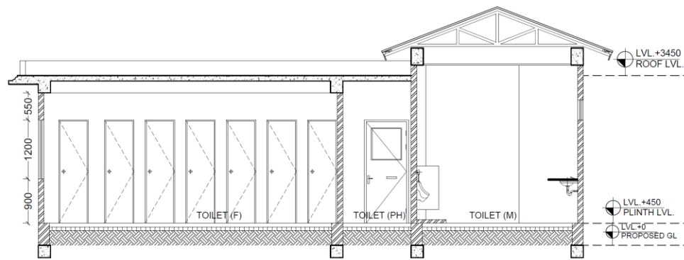
SECTION XX'
