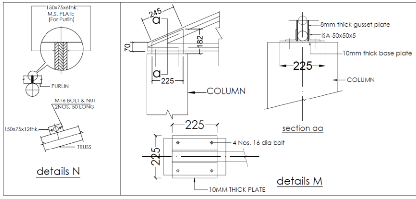
DETAILS - NTS ROOF TRUSS DETAILS
